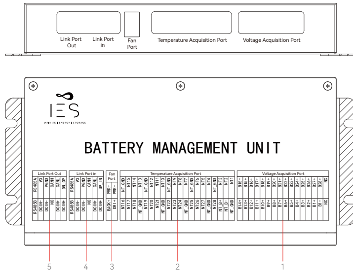
Figure 2.4 BMU photo
