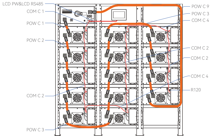
Wiring diagram
