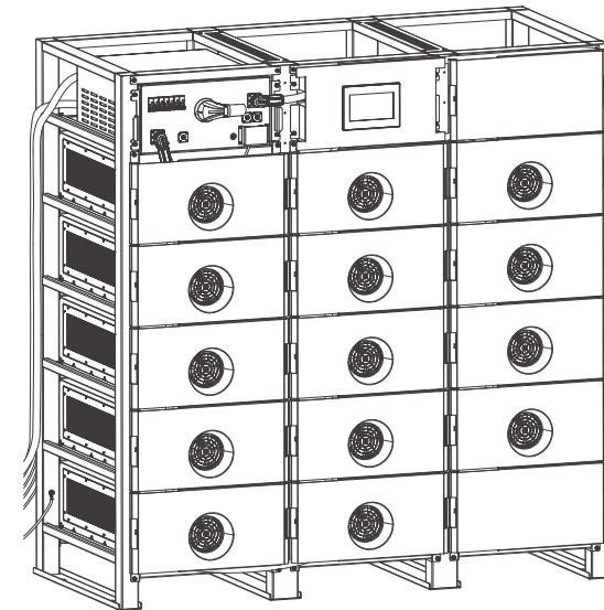
Figure 2.21 Overall diagram
