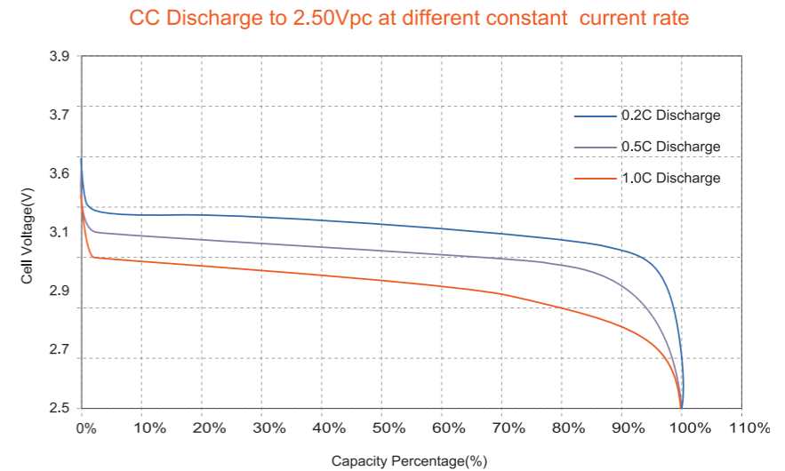
Fig.2-1 Discharge curve at different constant current of NPFC series
